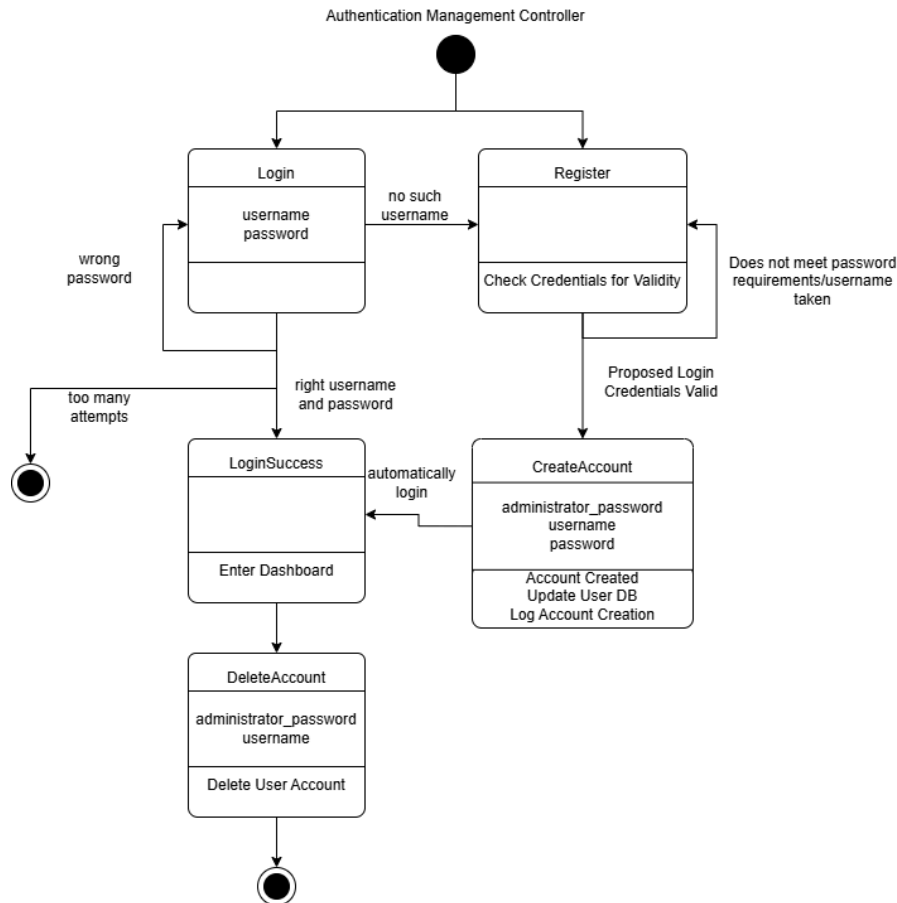
Figure 2.3. Authentication Management Controller State Diagram
