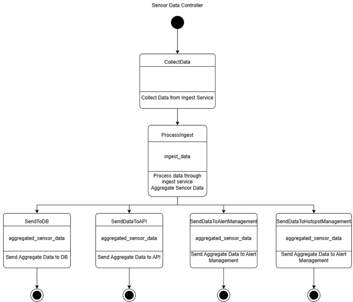
Figure 2.8. Sensor Data Controller State Diagram
