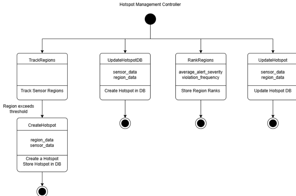
Figure 2.4. Hotspot Management Controller State Diagram
