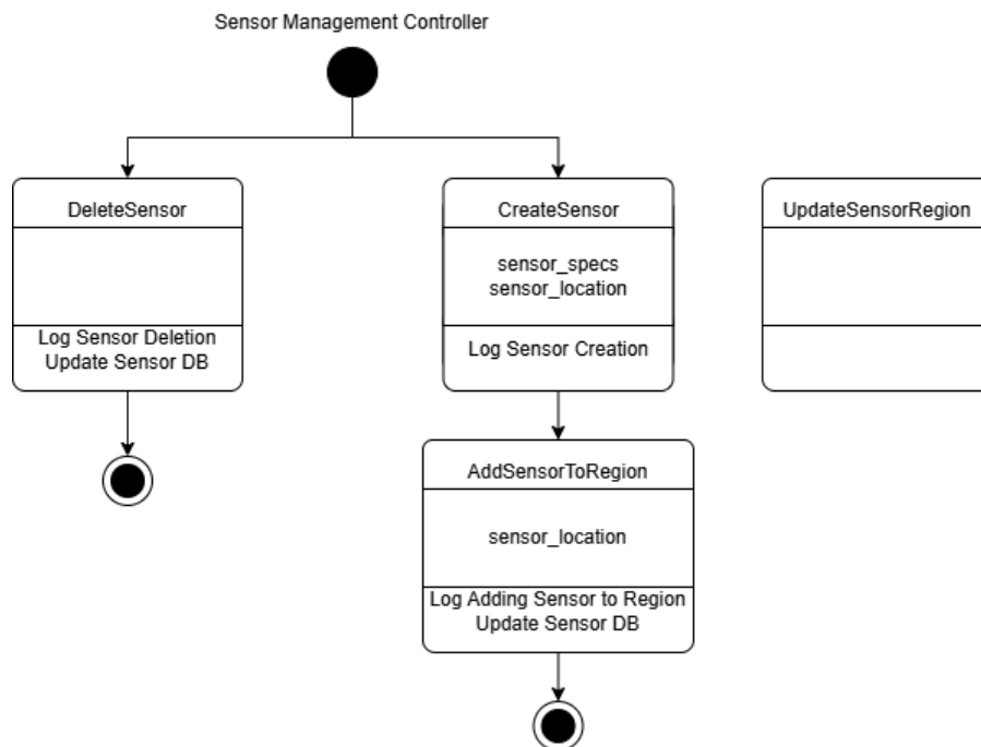
Figure 2.2. Sensor Management Controller State Diagram
