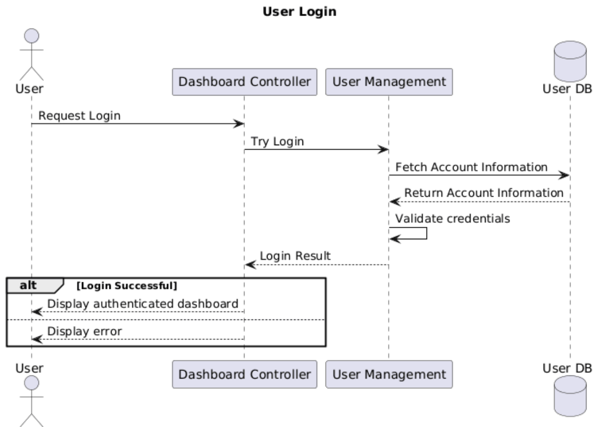
Figure 3.1. User Login Sequence Diagram
