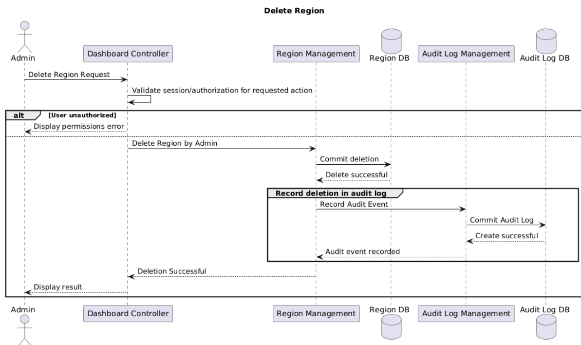
Figure 3.2. Delete Region Sequence Diagram
