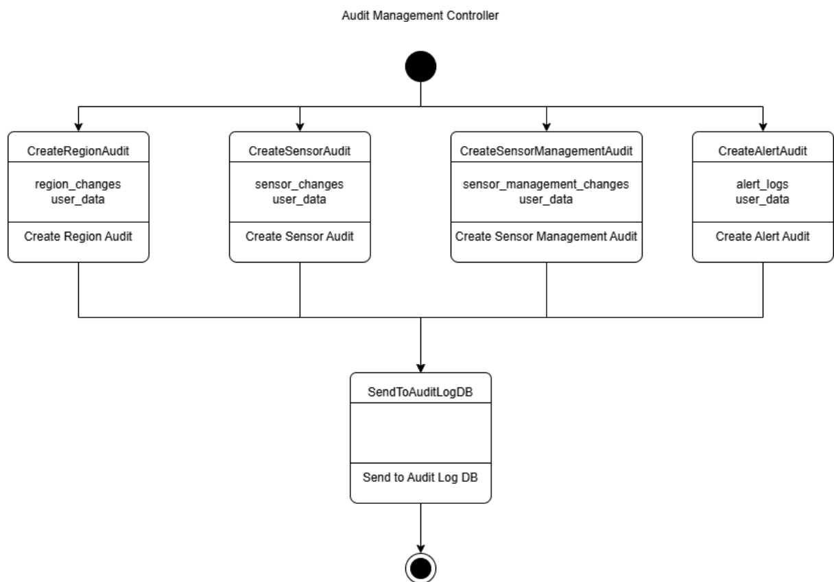
Figure 2.6. Audit Management Controller State Diagram
