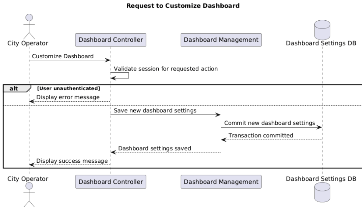
Figure 3.3. Dashboard Customization Sequence Diagram
