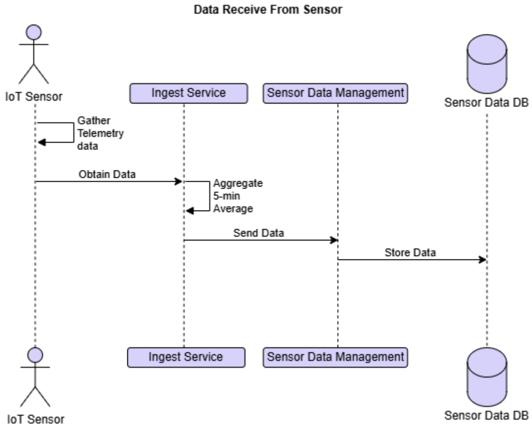
Figure 3.4. Data Receive From Sensor Sequence Diagram
