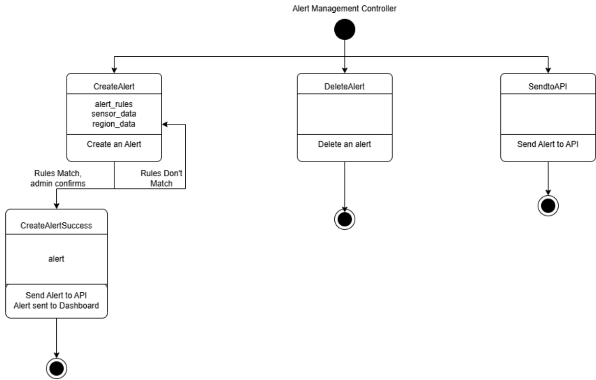
Figure 2.7. Alert Management Controller State Diagram
