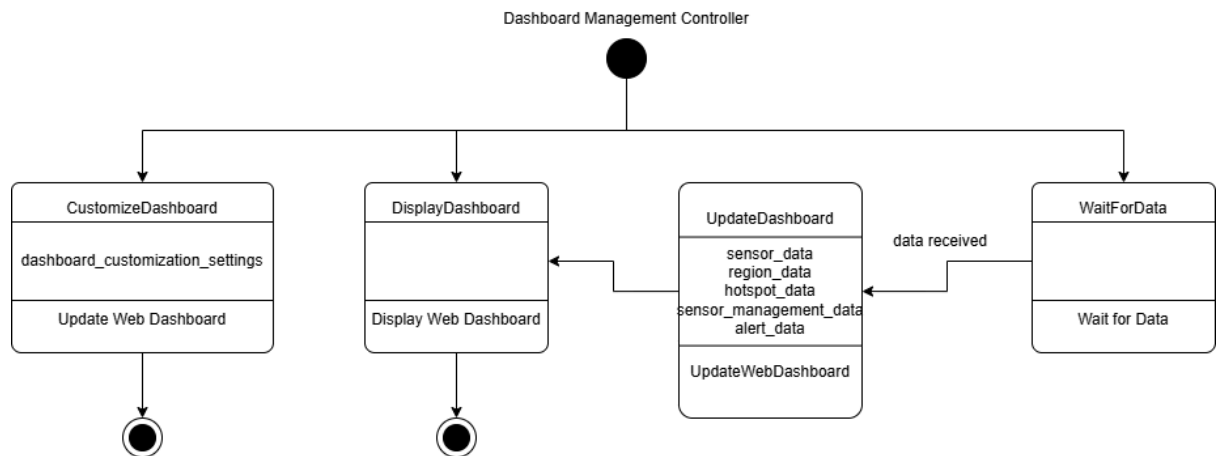
Figure 2.5. Dashboard Management Controller State Diagram
