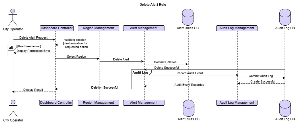
Figure 3.5. Delete Alert Rule Sequence Diagram
