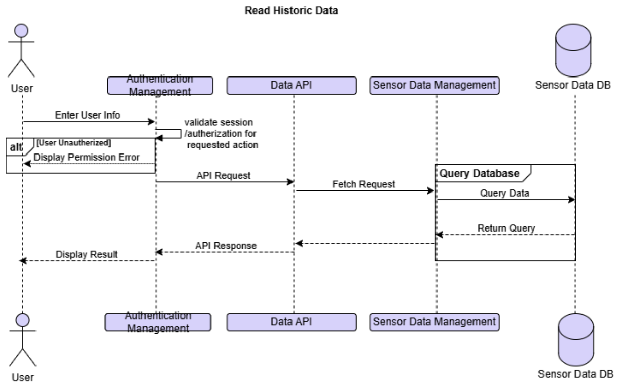
Figure 3.6. Read Historic Data Sequence Diagram
