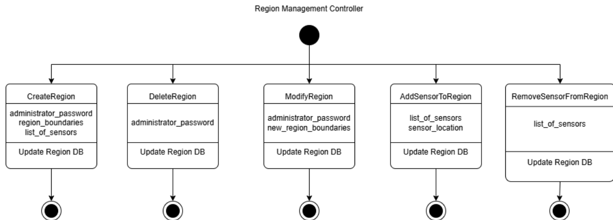
Figure 2.1. Region Management Controller State Diagram
